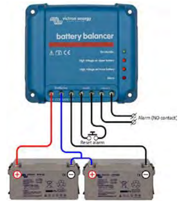
Battery Balancer (BMS012201000)
