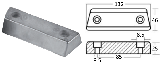
Base anode for Duo Prop foot
