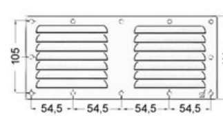
▲ 53.021.03/09
