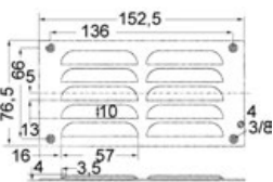
▲ 53.021.05/11
